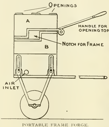
PORTABLE FRAME FORGE.
